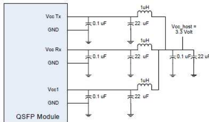
Figure 4. Recommended Host Board Power Supply Filter Network
